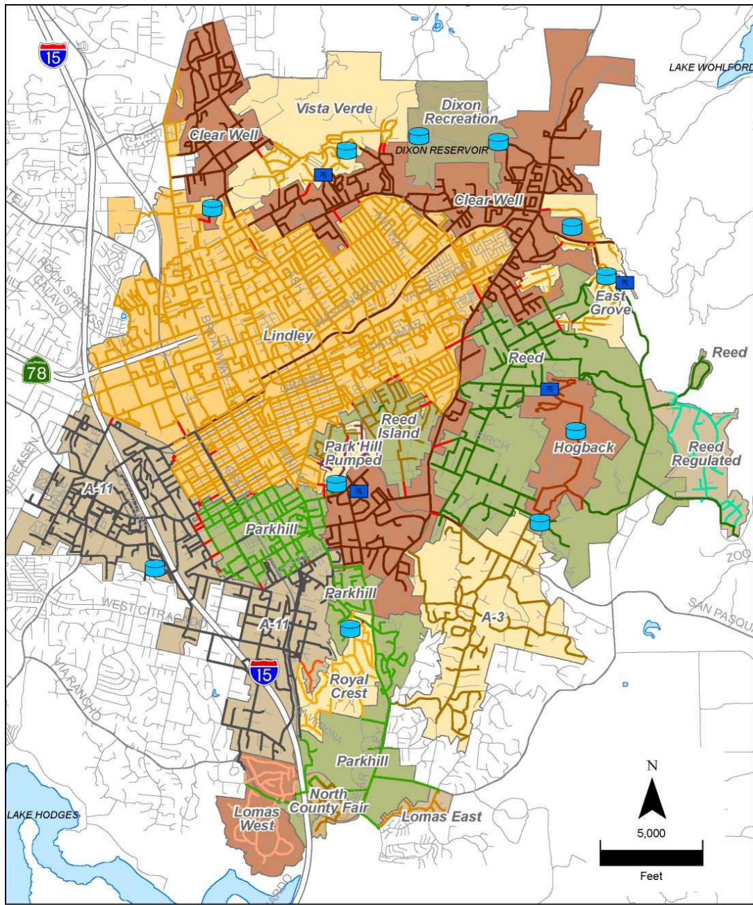
Water Pressure Zones
