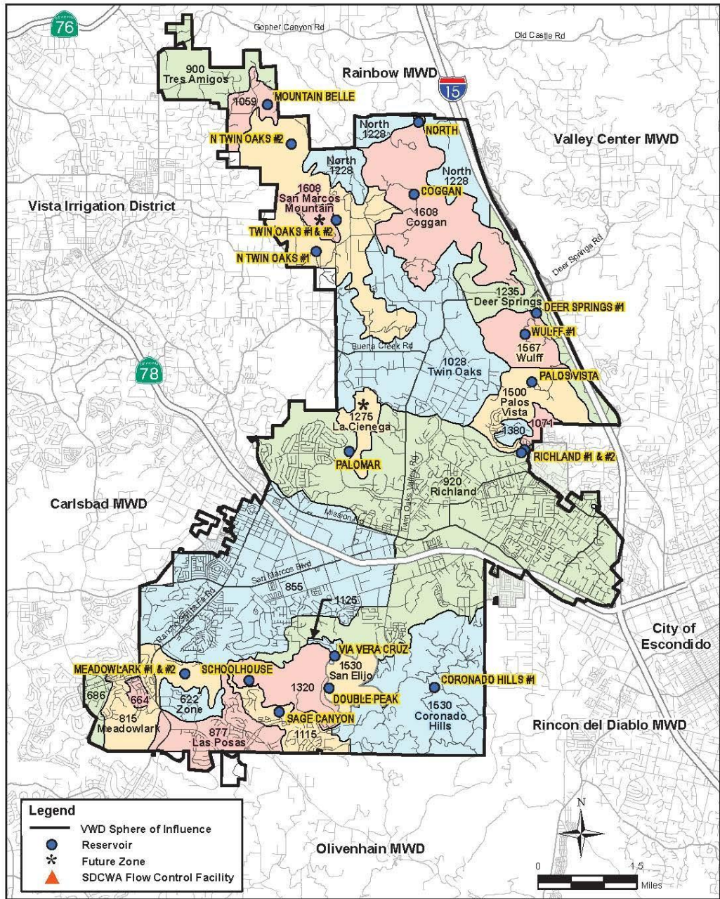
Figure 13-2 Vallecitos Water Facilities
