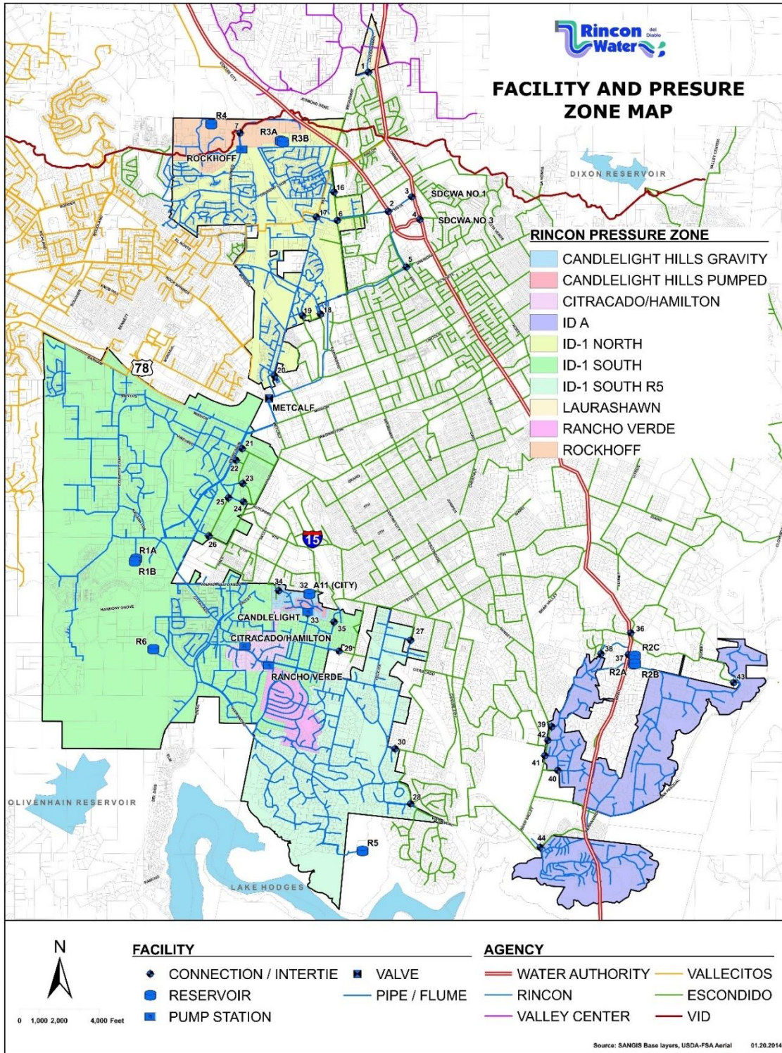
Figure 10-2 Rincon Water Facilities
